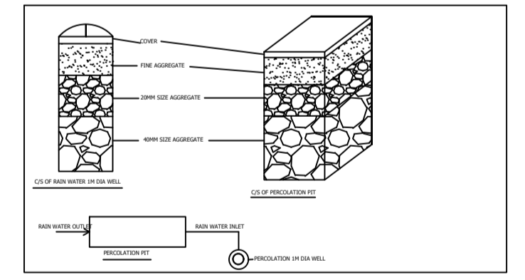
DETAILS OF RAIN WATER HARVESTING
